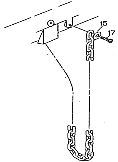
Lower Hook Assembly AH-25C, AH-50C
